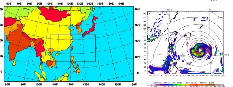
Domains of CWB-WRF OP4.0
